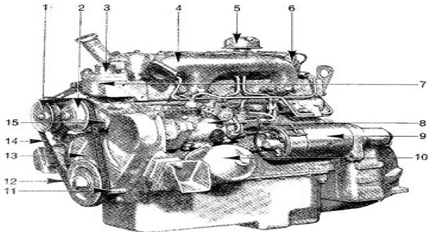
VIEW OF FUEL PUMP SIDE OF ENGINE
