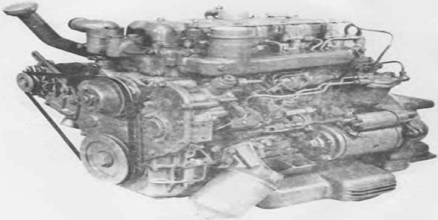
View of Front Left Head Side of 4, 154 Engine
