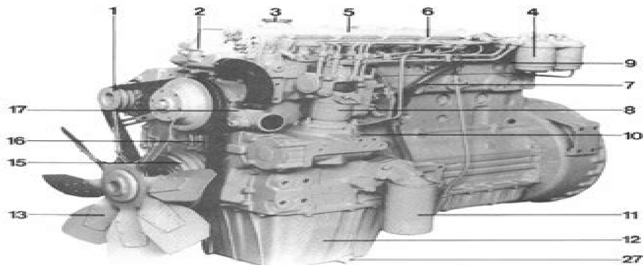
A.1 View of Fuel Pump Side of 6.3544 Engine
