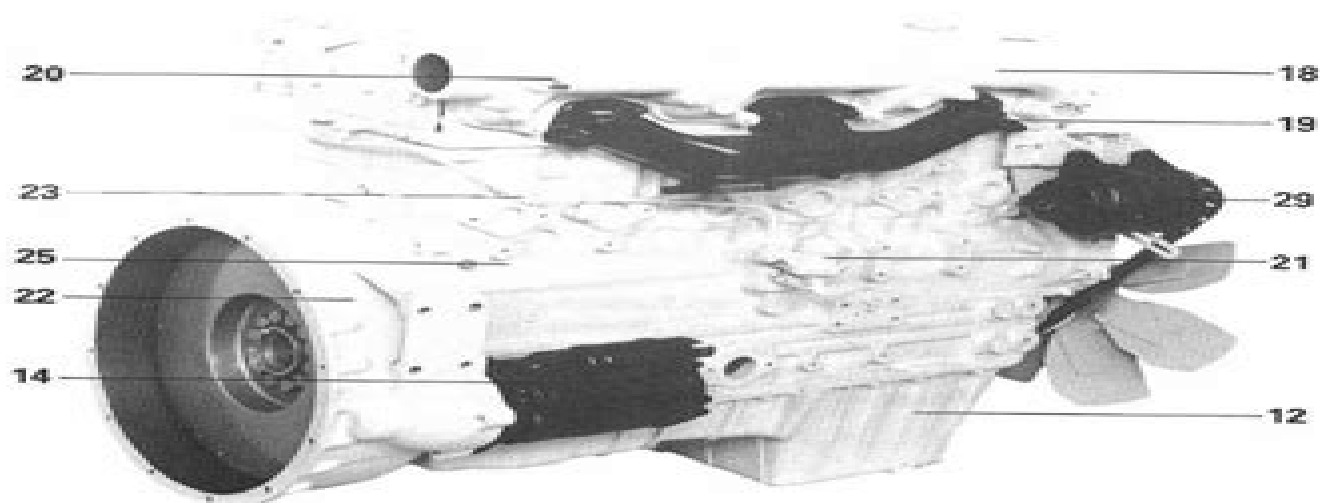
A.2 View of Camshaft Side of 6.3544 Engine
