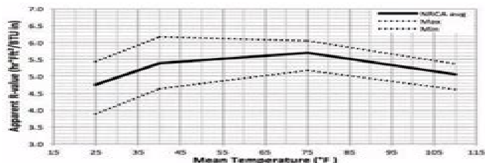
Figure 2: NRCA examined R-value minimum and maximum ranges for polyisocyanurate samples.
