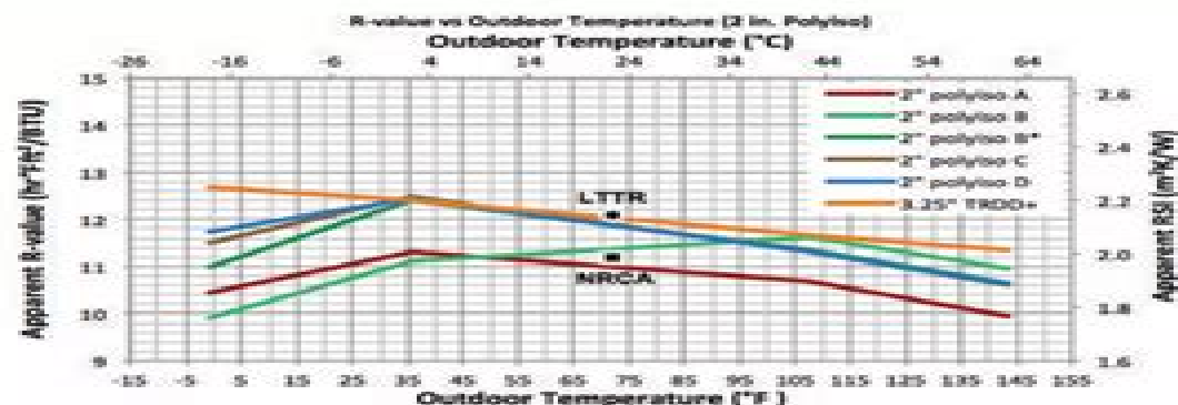
Figure 1: BSCI tested the apparent R-value on four polyisocyanurate manufacturers' samples, including a sample of high-density mineral wool roofing material. LTTR stands for long-term thermal resistance; NRCA represents that organization's testing results.
