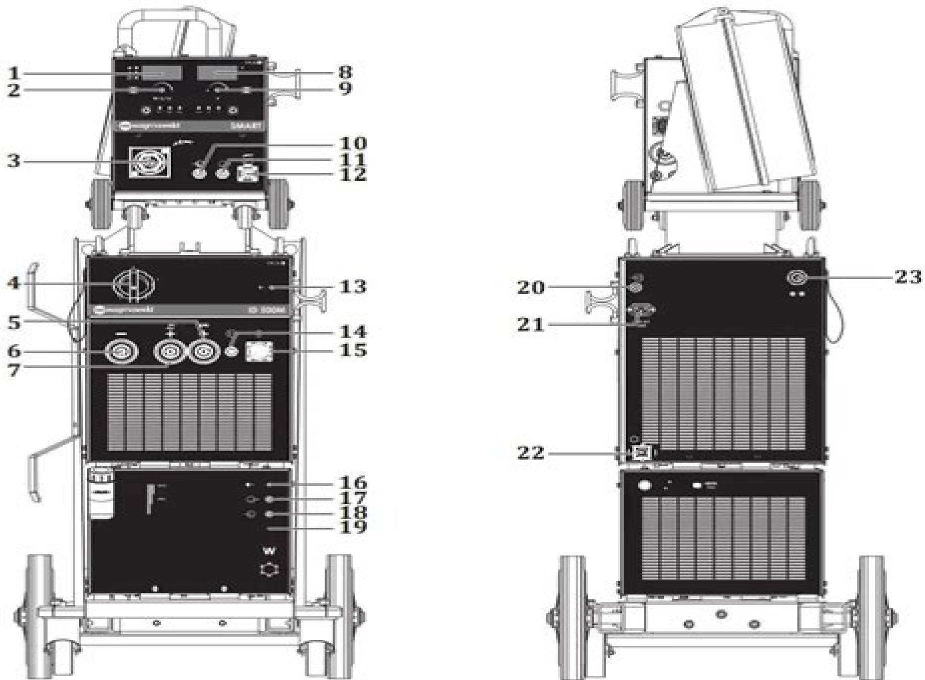
Figure 2 : ID 500 MW SMART - ID 500 MW PULSE SMART Front and Rear View
