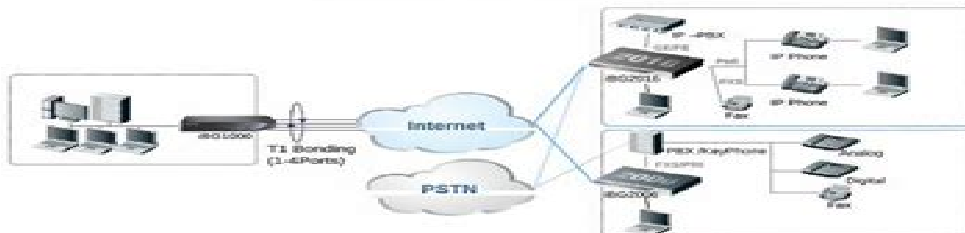
Ubigate iBG1000 Deployment with T1 multi-link bonding
