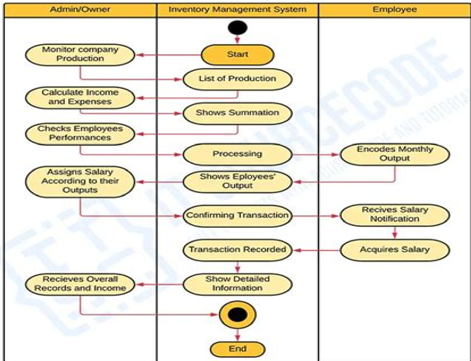
ACTIVITY DIAGRAM
