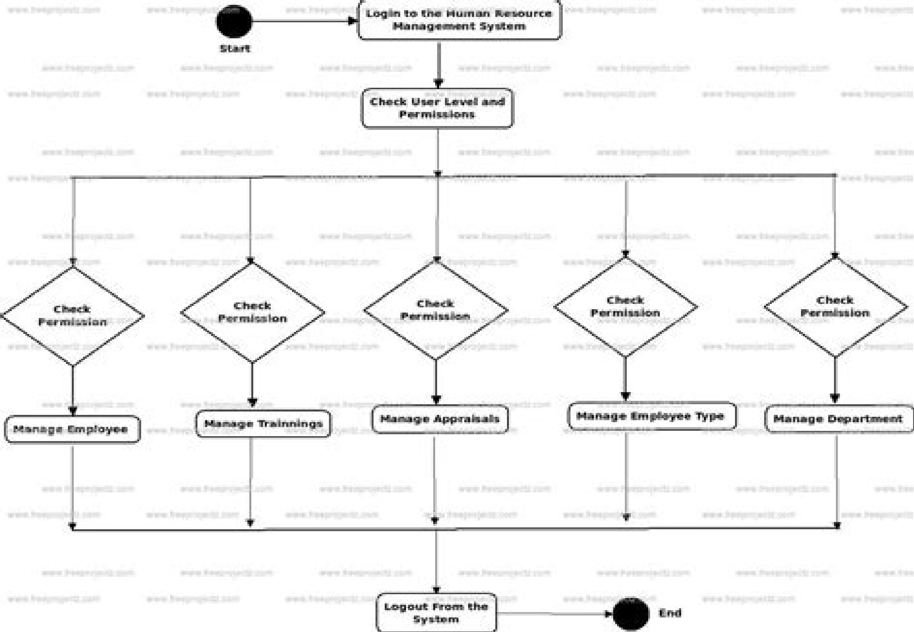
Activity Diagram for Human Resource Management System
