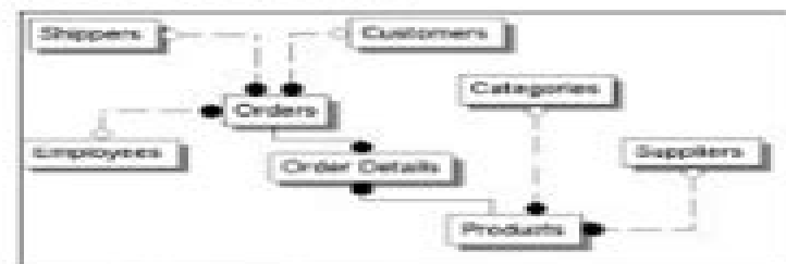
Figure 1. Main subject Access ERD
