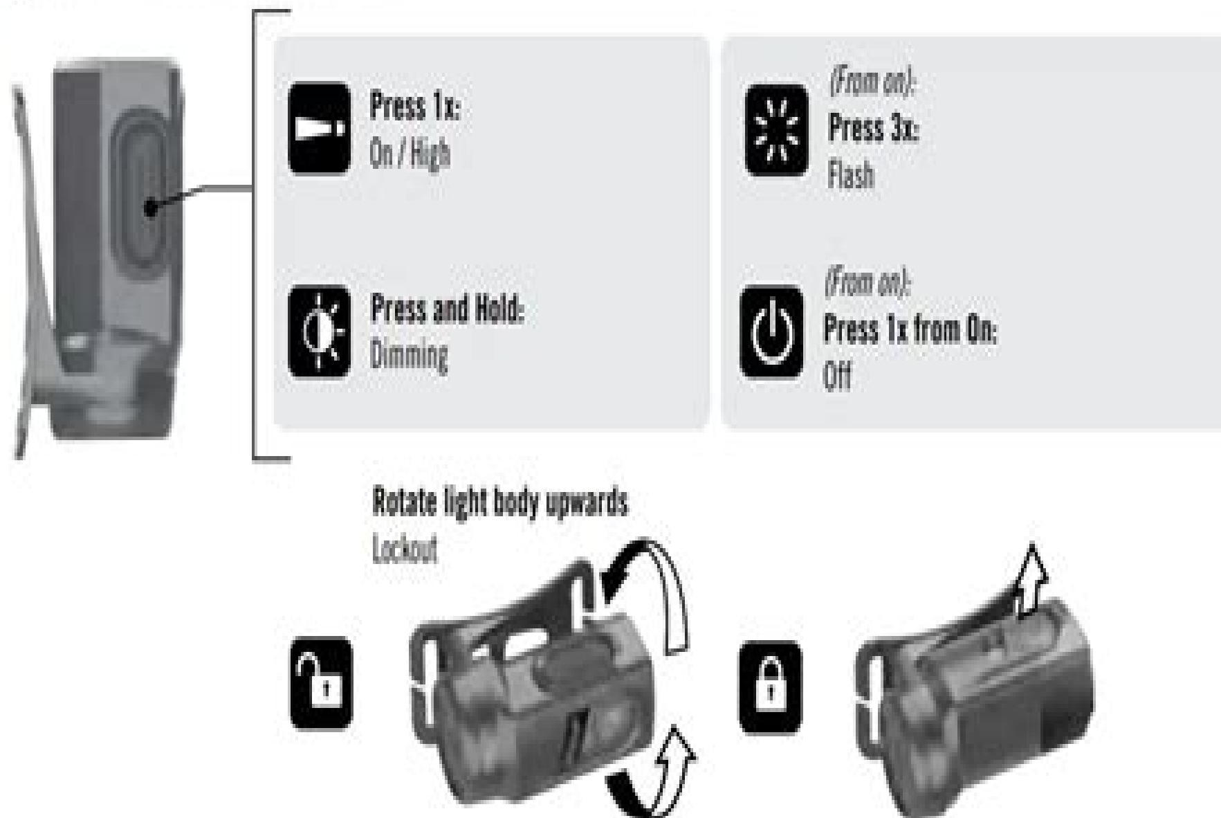
Figure 2 – Switch Operation
