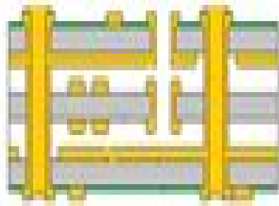
Multi-Sided PCB
