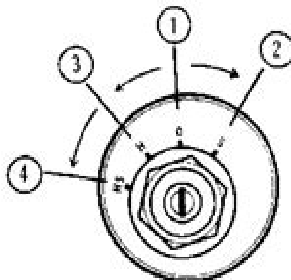
Fig. 2. Combined Hand/Start Switch 1 Off Position 3 Stop Position 2 Run Position 4 Start and Run Position
