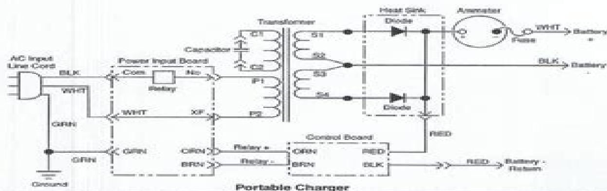
Fig. 5 PowerWise™ Charger Wiring Diagrams
