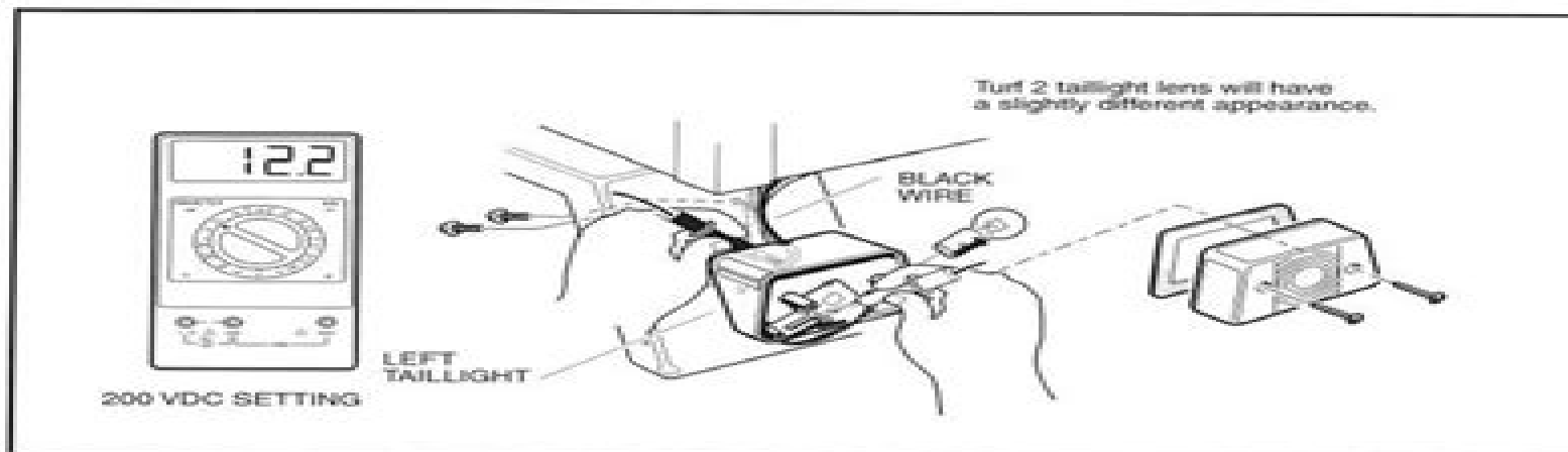
Figure 11-48 Taillight Socket Voltage Test
