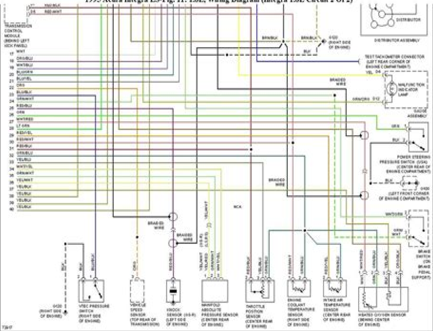
1995 Acura Integra LS-Fig. 11: L&L, Wiring Diagram (Integra L&L Circuit 2 Of 2)
