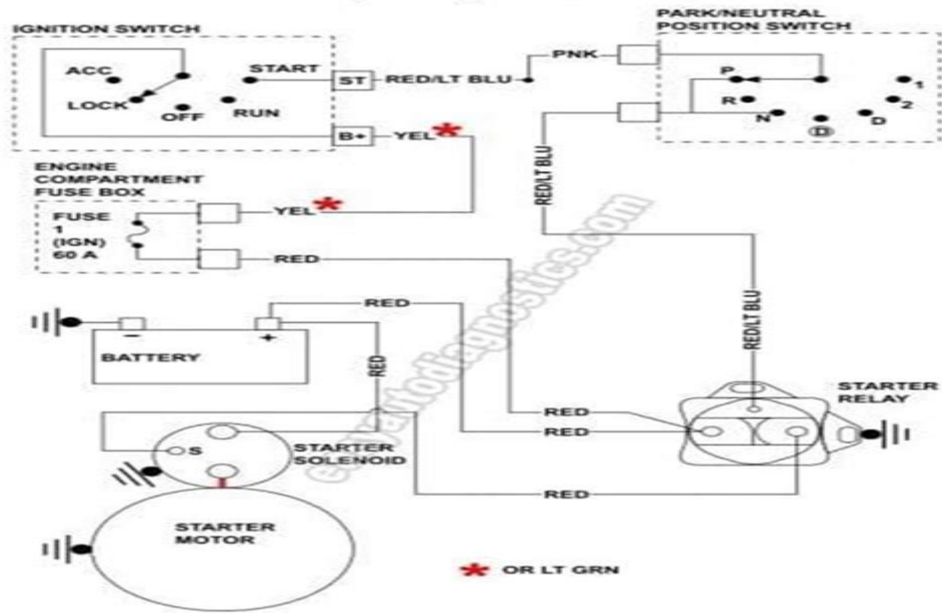
STARTER MOTOR WIRING DIAGRAM (A/T) (1992-94 4.0L V6 EXPLORER - RANGER)
