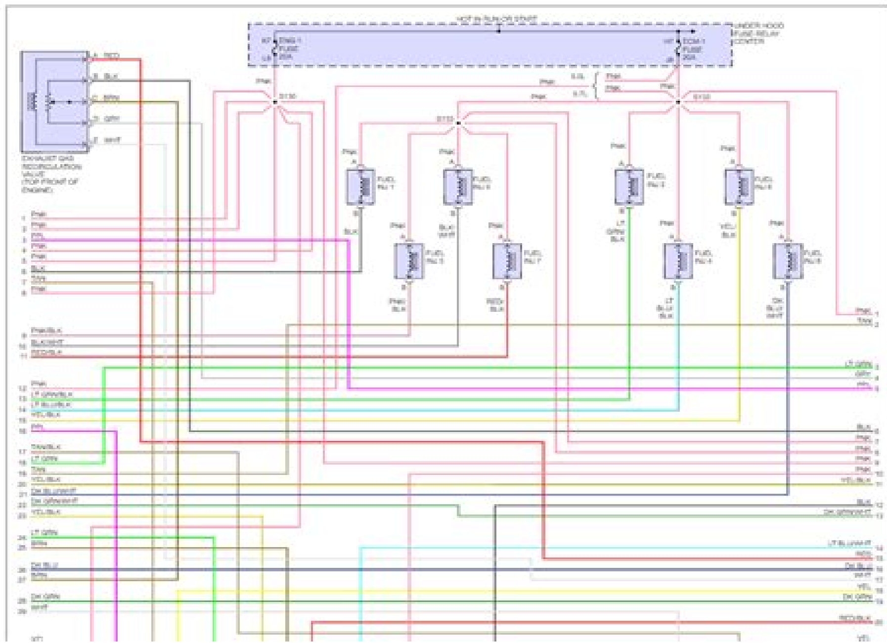
Fig 2: 5.7L VIN R, Engine Performance Circuits (2 of 4)
