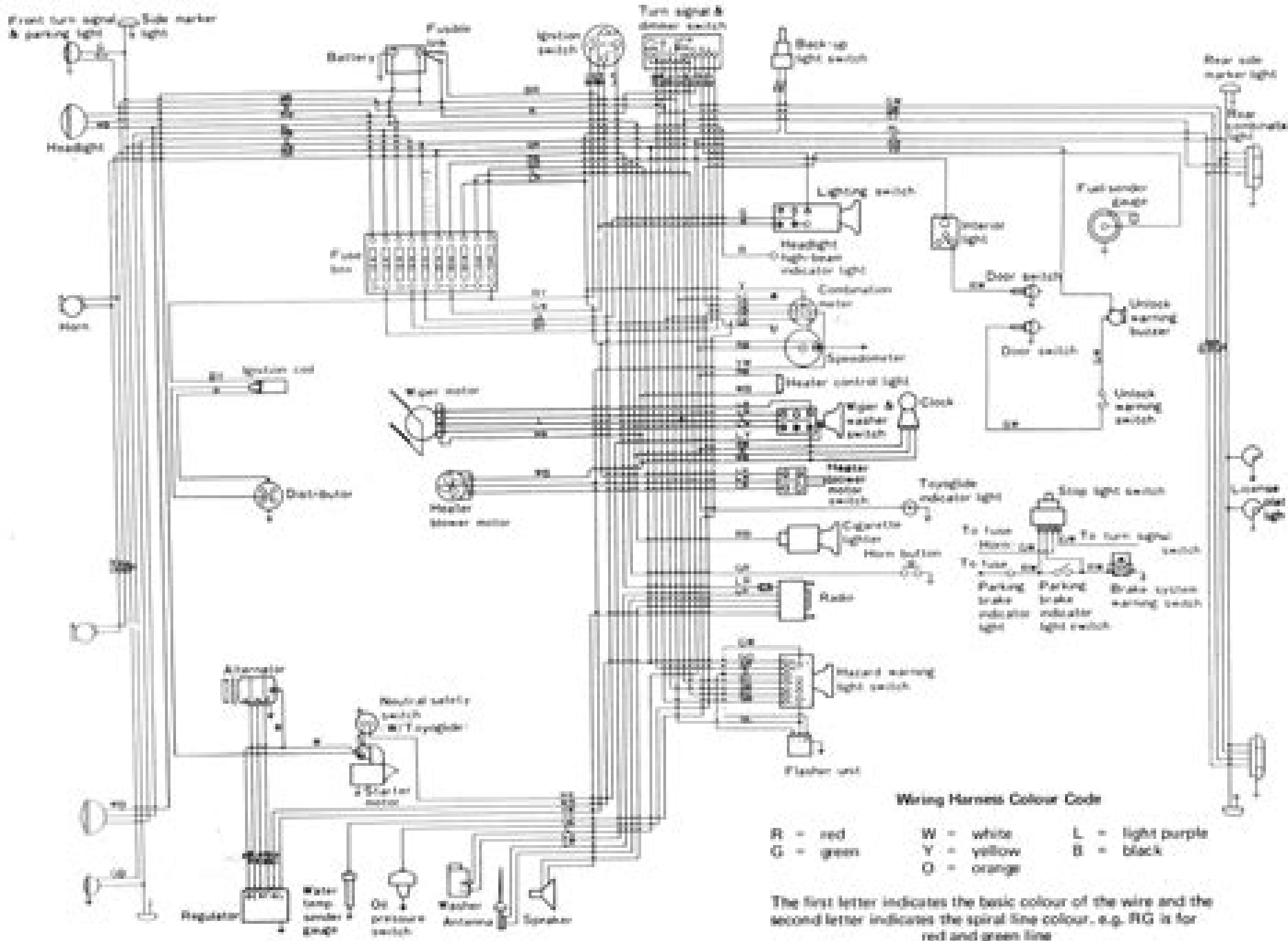
Wiring diagram – USA KE and TE models
