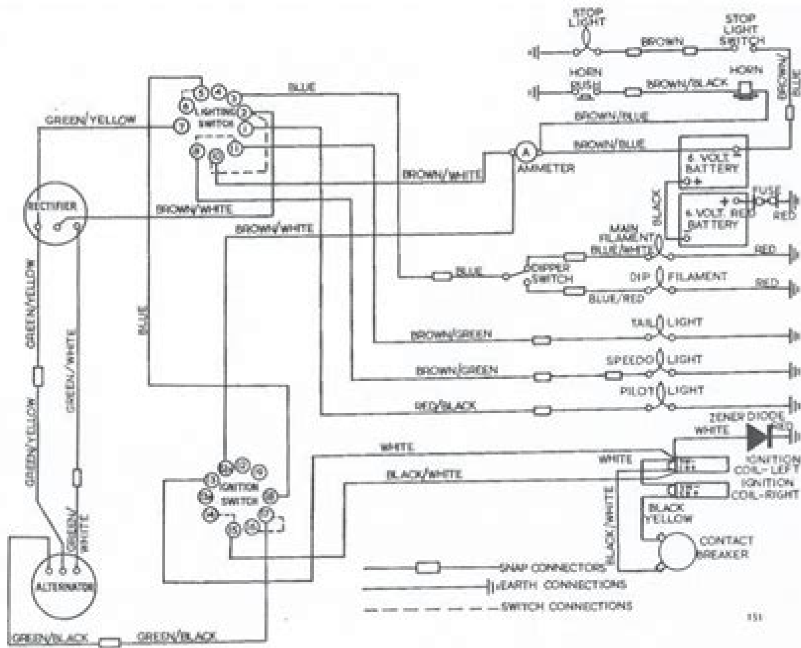
Fig. H31. Wiring diagram—Coil ignition 12V models with 2ener Diode and 3 rate charge control Before engine number DU 24875
