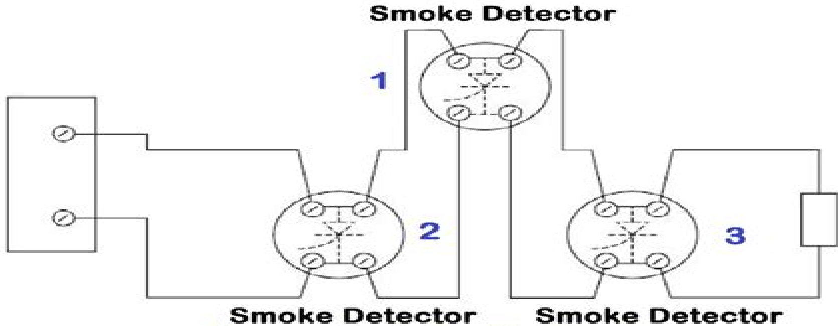
Correct wiring Method
