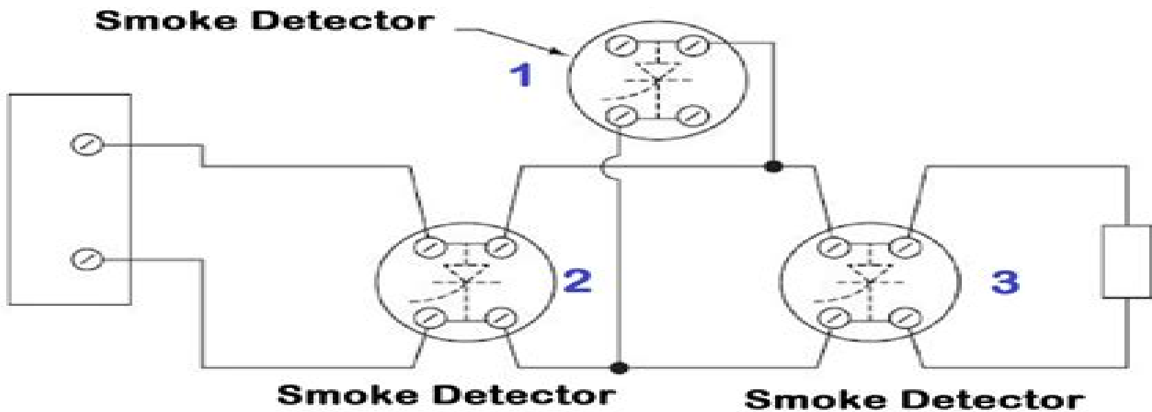
Incorrect Wiring Method
