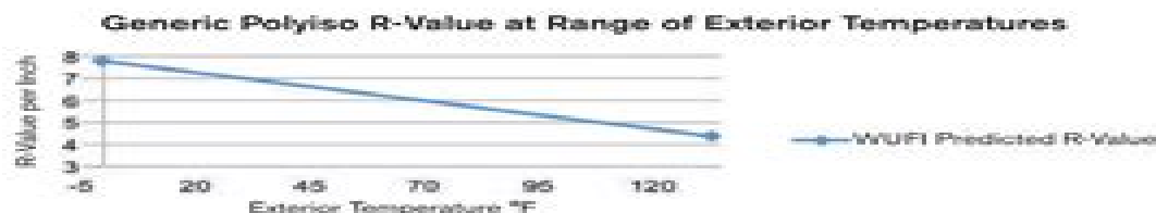
Figure 4: The WUFI-ORNL/IBP 5.3 database predicted the R-value of polyisocyanurate.
