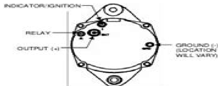
21SI, 22SI & 23SI NON-REMOTE SENSE (23SI TERMINAL LOCATIONS VARY)
