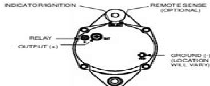
21SI & 22SI REMOTE SENSE 2-TERMINAL REGULATOR
