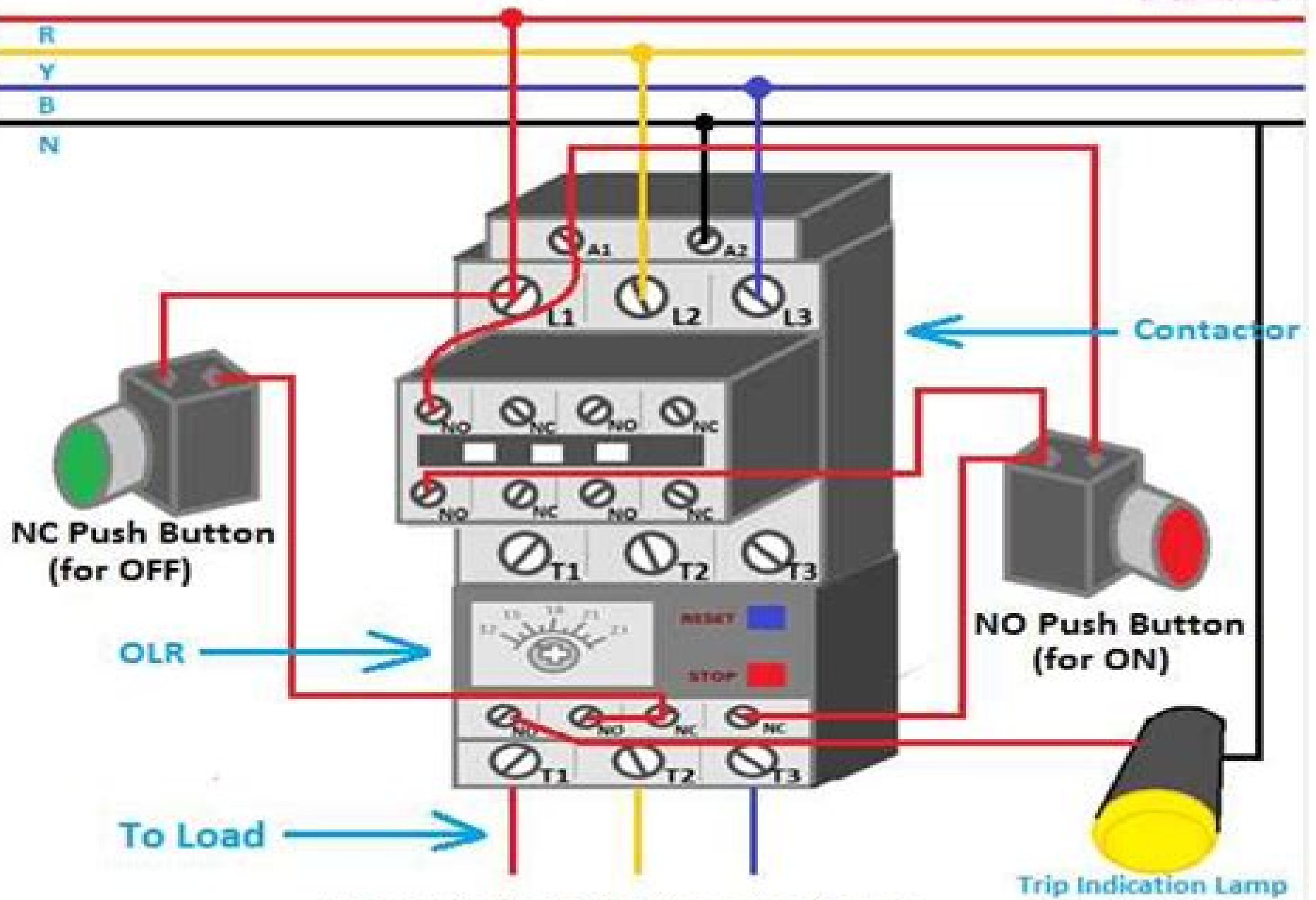
Thermal Overload Relay Connection Diagram
