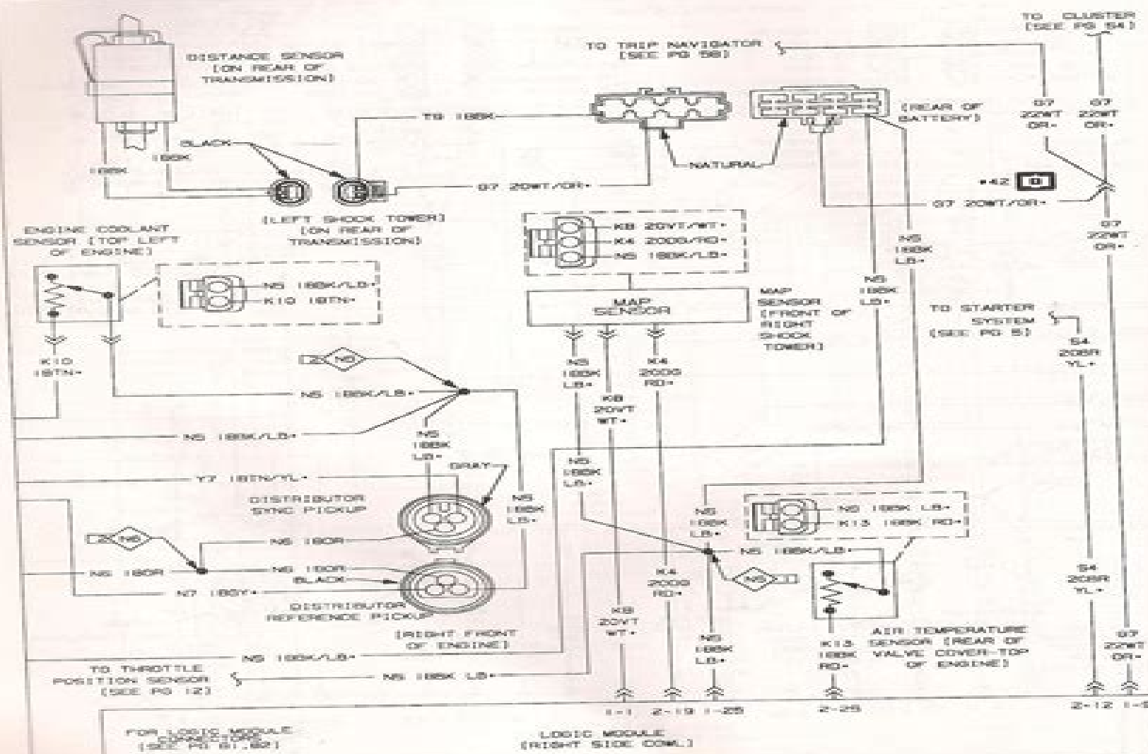
TURBOCHARGED ELECTRONIC FUEL INJECTION IGNITION SYSTEM
