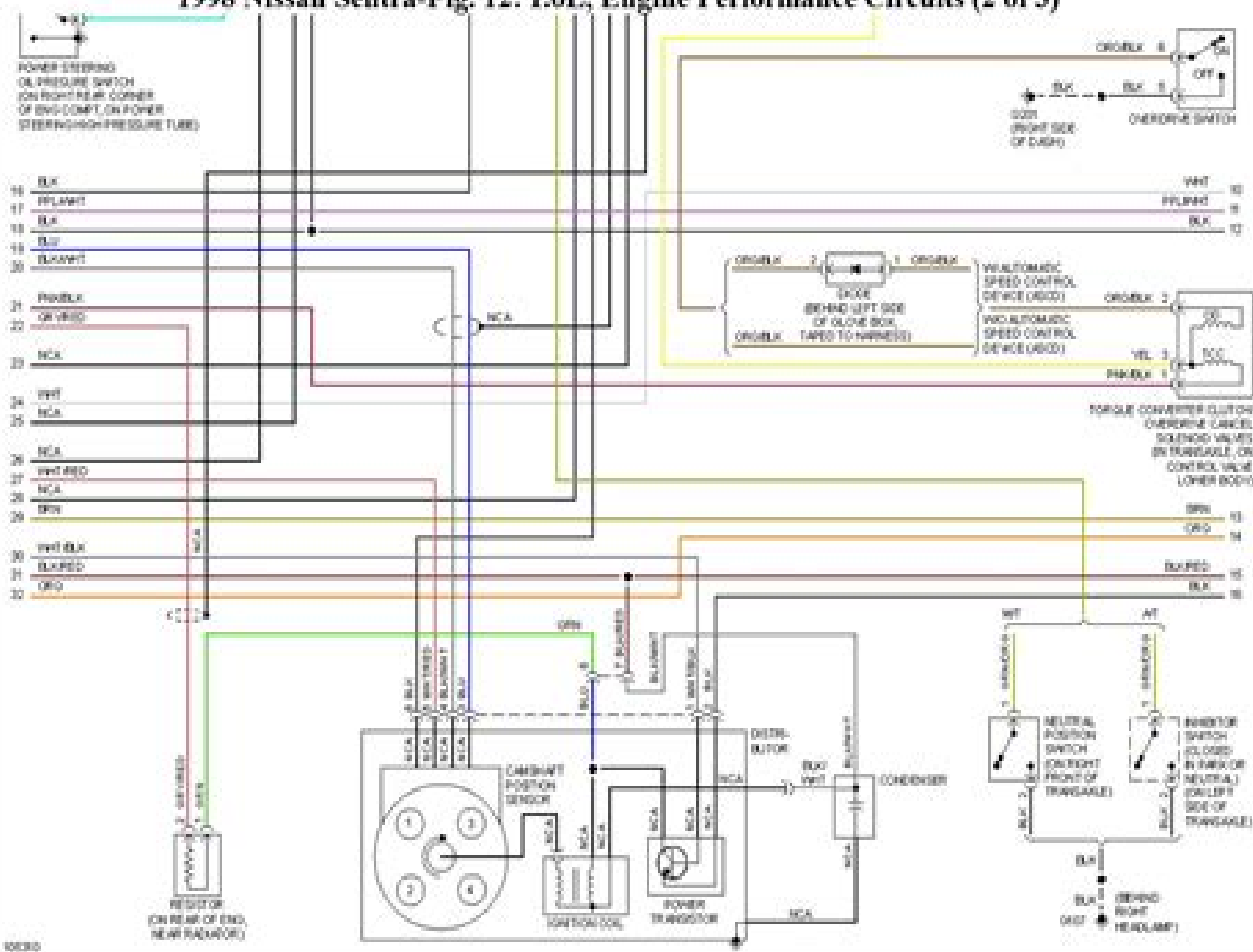
1998 Nissan Sentra-Fig. 12: 1.6L, Engine Performance Circuits (2 of 3)
