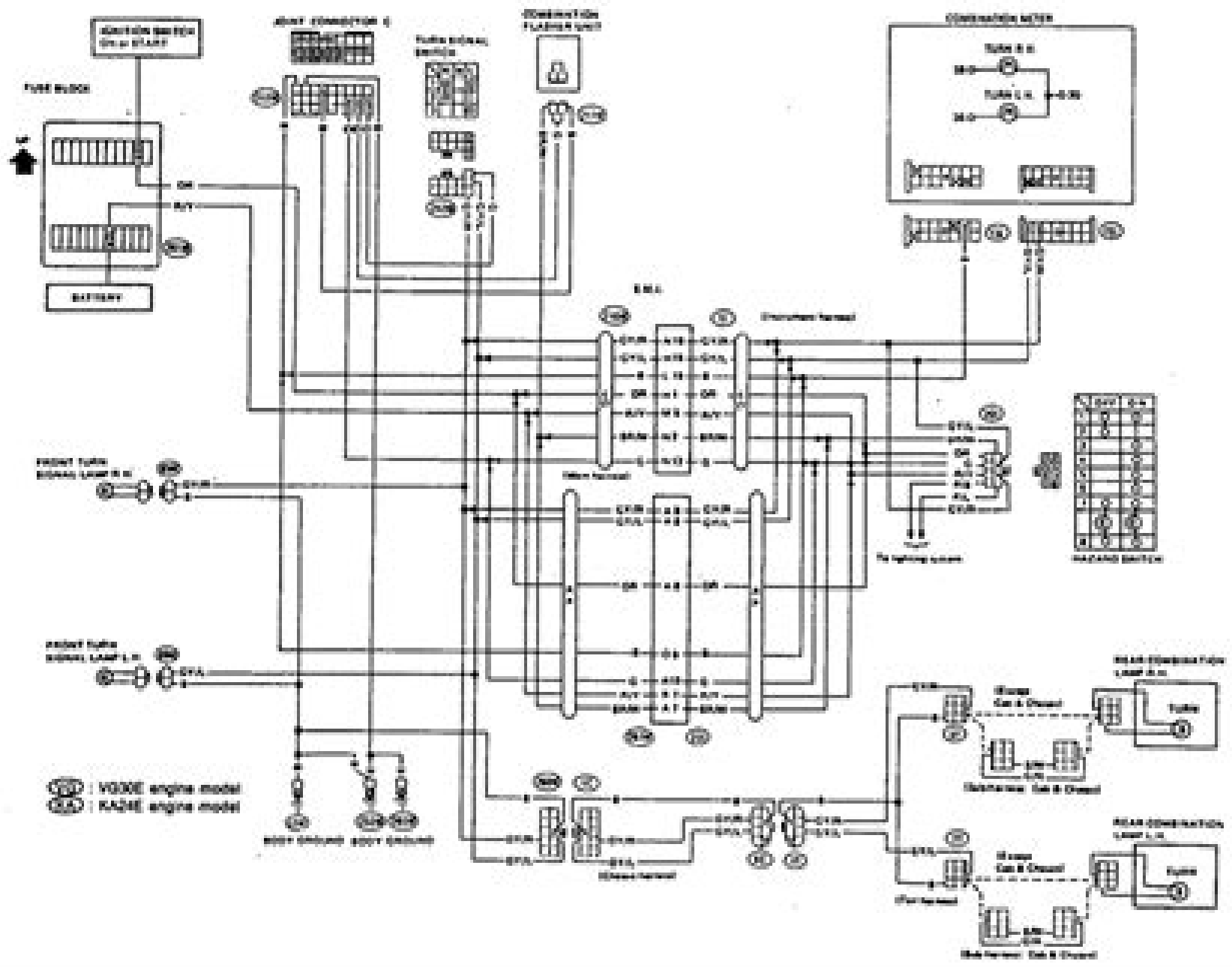
Diagram 1 Combination Flasher Unit
