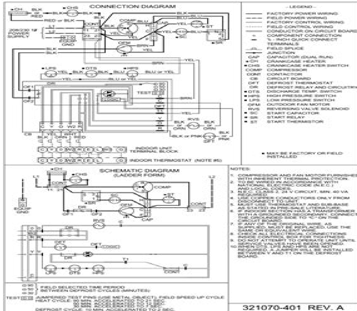
Fig. 1—38YCA018 (331, 341), 38YCA/YN024 (351,361), 38YCA/YN030 (361,371), 38YCA/YN036 (371) 208-230v, 1 Phase, 60 Hertz
