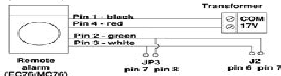
Figure 3. Remote alarm wiring (multiple pedestals)
