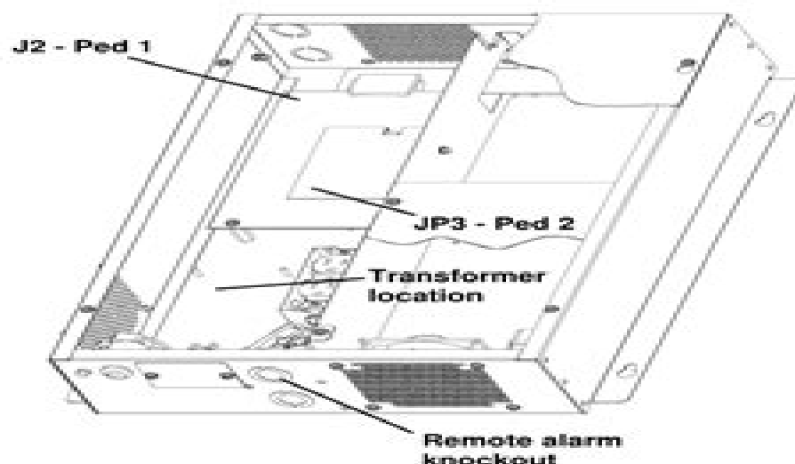
Figure 4. Transformer and remote alarm connection
