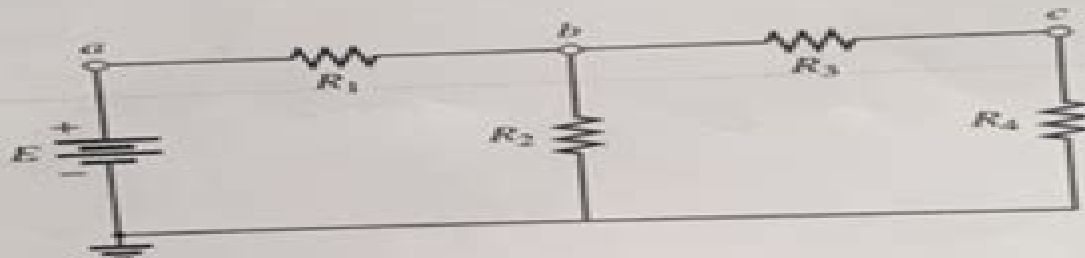
FIG. 7.1 Series-parallel dc network.
