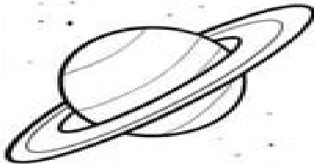
SATURN
