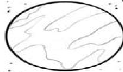
MERCURY
