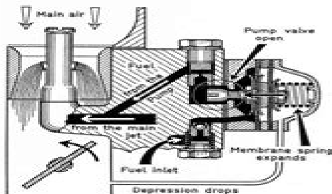
Fig. 30 Depression-operated accelerator pump
