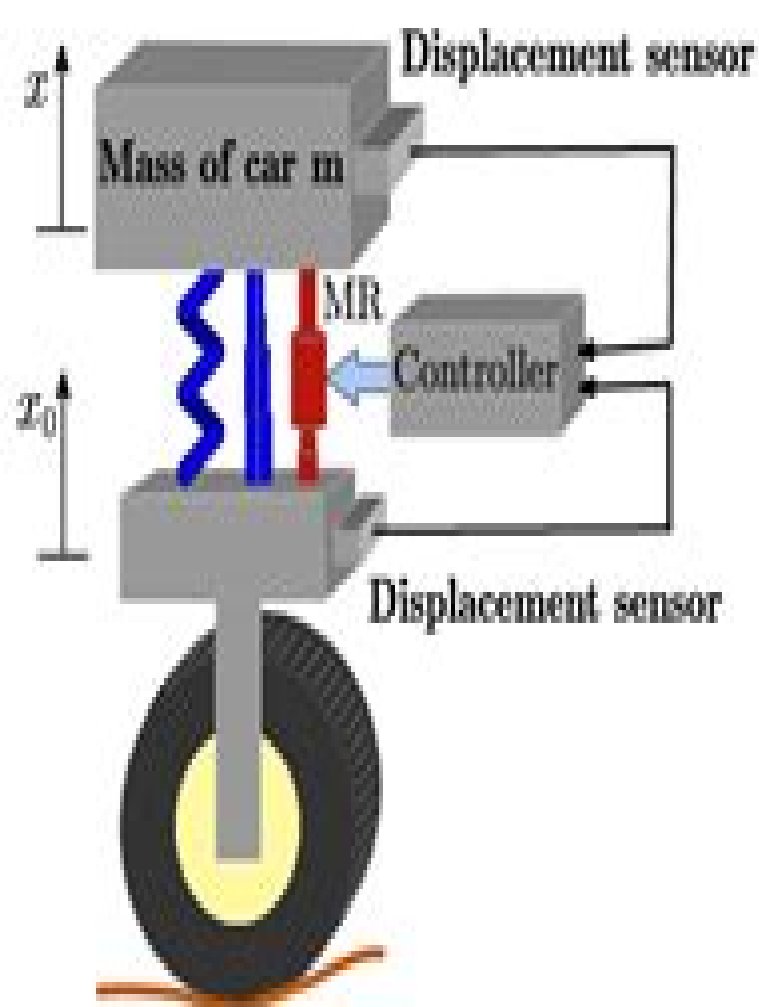
b) Active suspension
