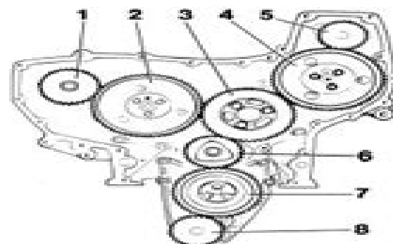
Timing gear
