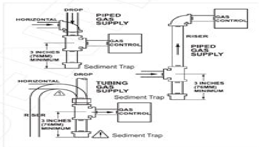
Figure 9: Sediment Trap (where required)
