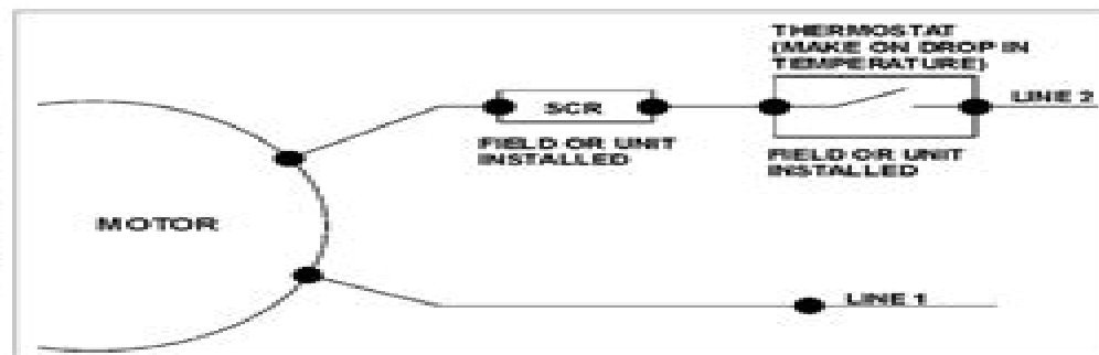
FIGURE 1 MOTOR WIRING DIAGRAM
