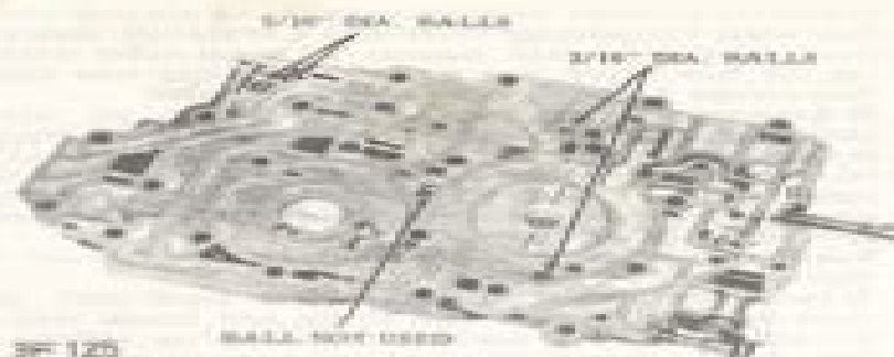
1962-63 CHECK BALLS (CHANNEL PLATE)
