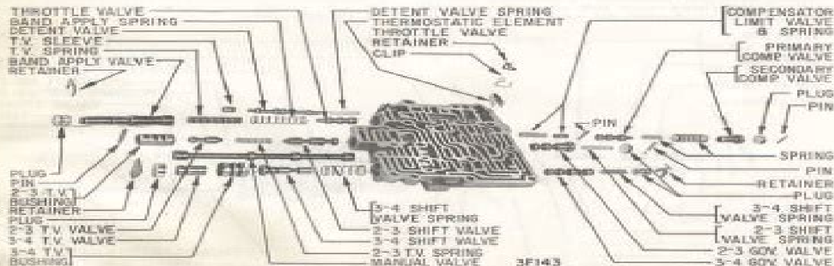
1962-63 PRIMARY VALVE BODY ASSEMBLY
