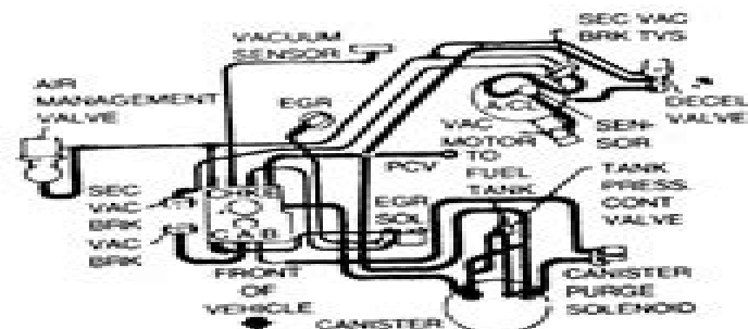
FIG. 5: 1984 2.5L CARBURETED; CANADA
