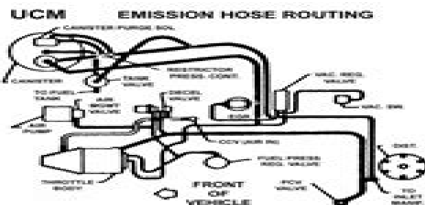
1985 2.5L FUEL INJECTED
