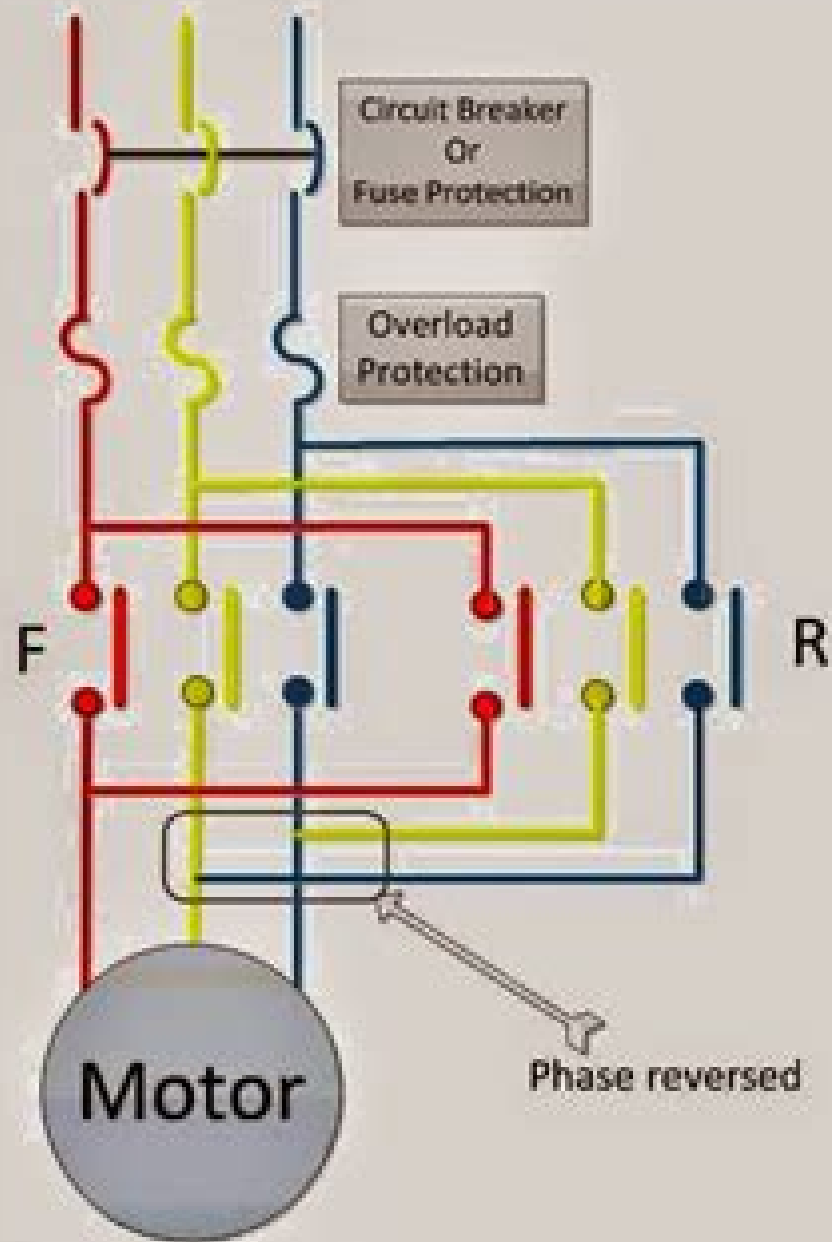
Power Circuit
