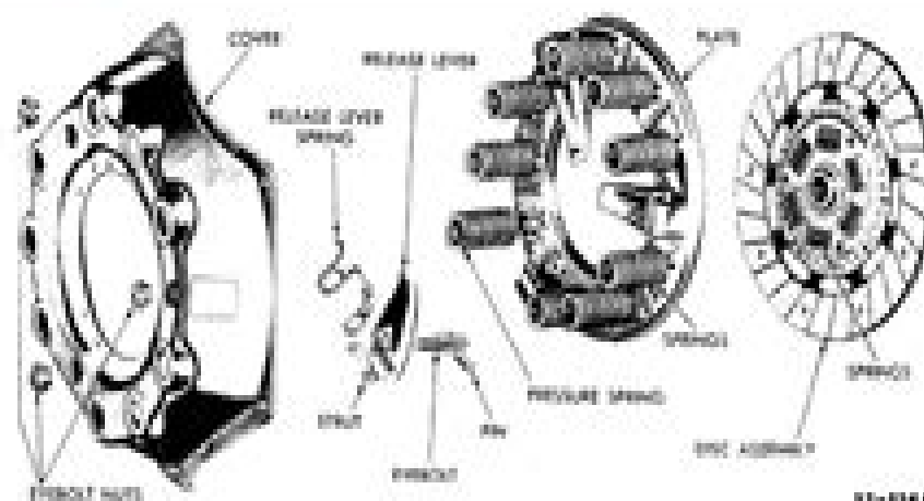
Fig. 1--Typical Clutch Assembly (Exploded View) (8-Cylinder Engine)
