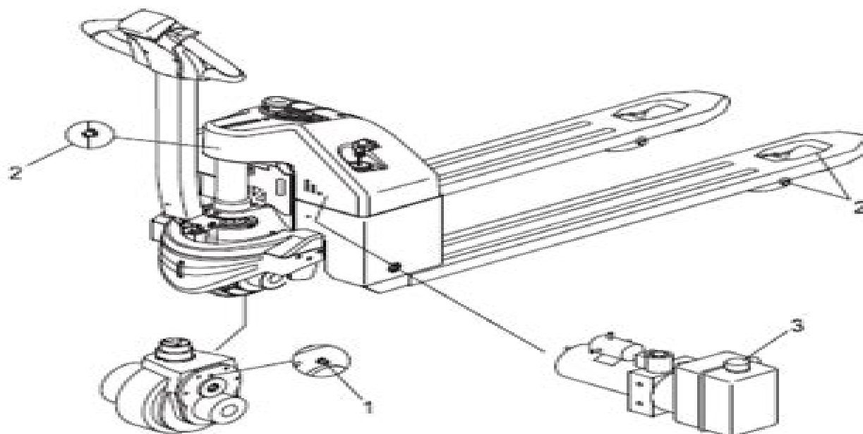
Figure 3-7 Lubrication Diagram
