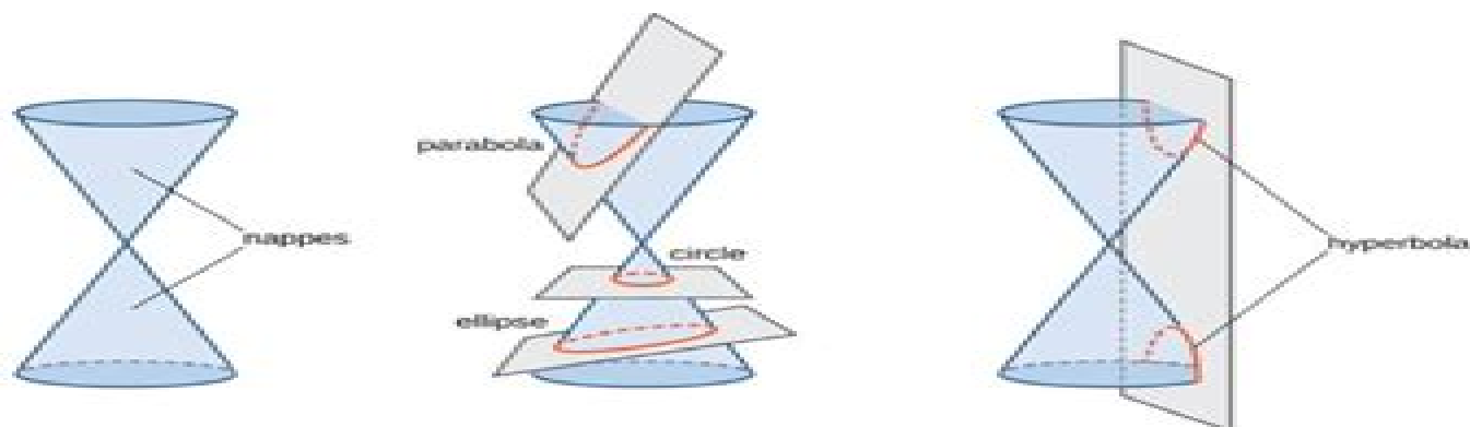
A cone and conic sections: The nappes and the four conic sections. Each conic is determined by the angle the plane makes with the axis of the cone.
