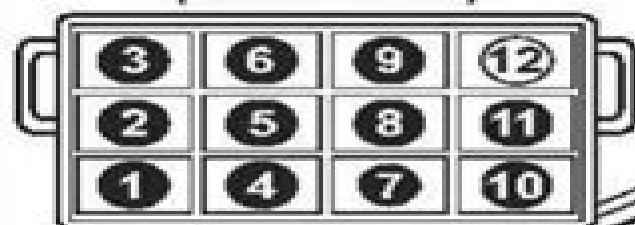
INPUT CONNECTOR (REAR VIEW)
