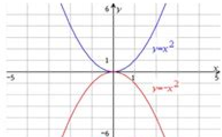
Reflected Across the X-Axis
