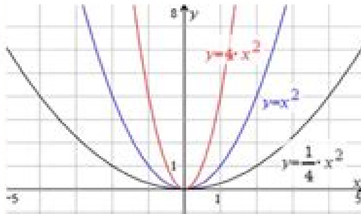
Horizontal Stretch ( Wider ) Vertical Stretch ( Narrower )
