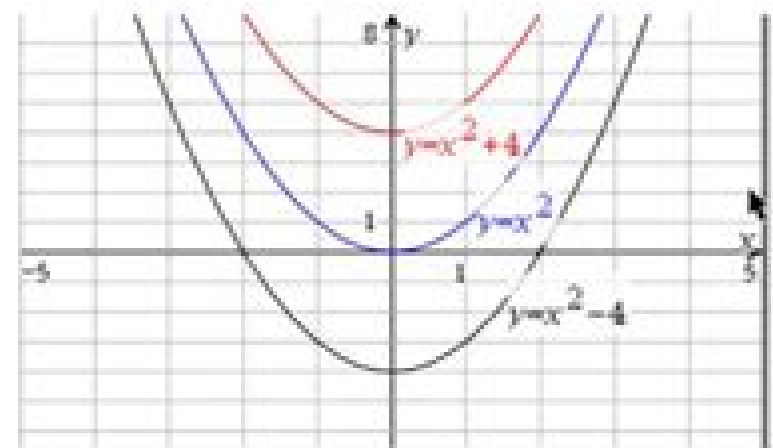
Vertical Shift ( Down ) Vertical Shift ( Up )
