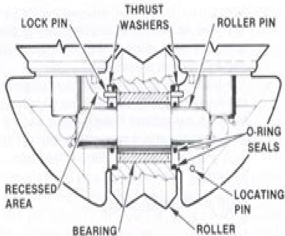
Kelly Bushing Roller Section
