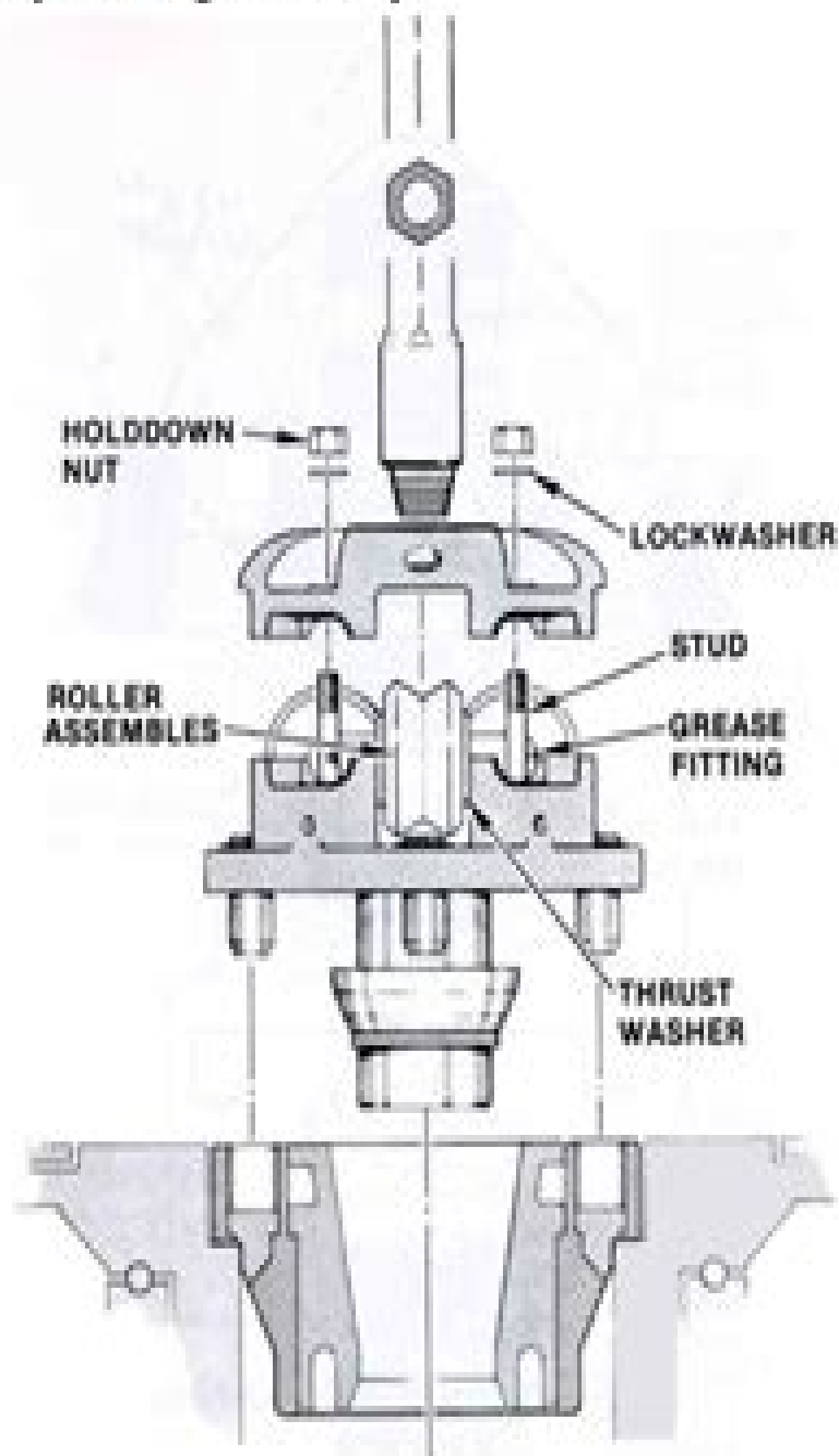
Kelly Bushing Assembly
