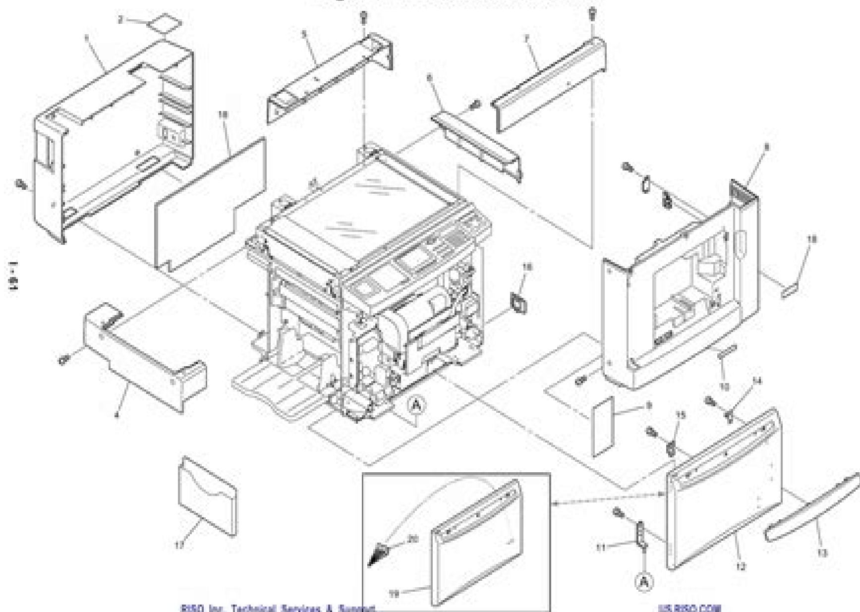
Fig.30 RN Exterior Cover Area
