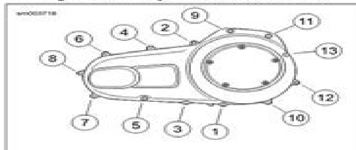
Figure 7-3. Primary Chaincase Cover Tightening Sequence
