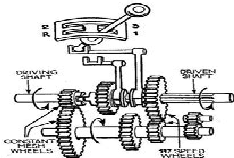
First speed engaged
