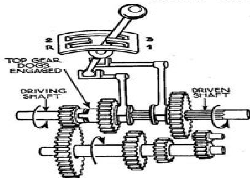
Third, or top : " dogs " are used
