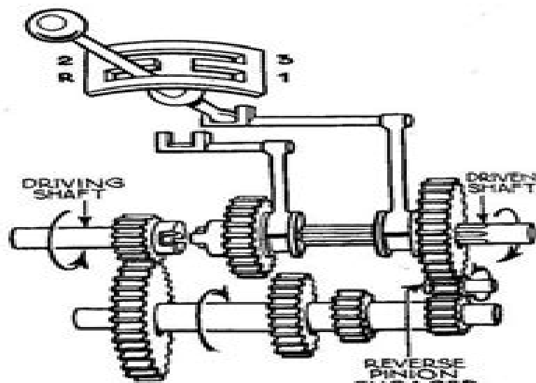
The separate reverse train of gears
