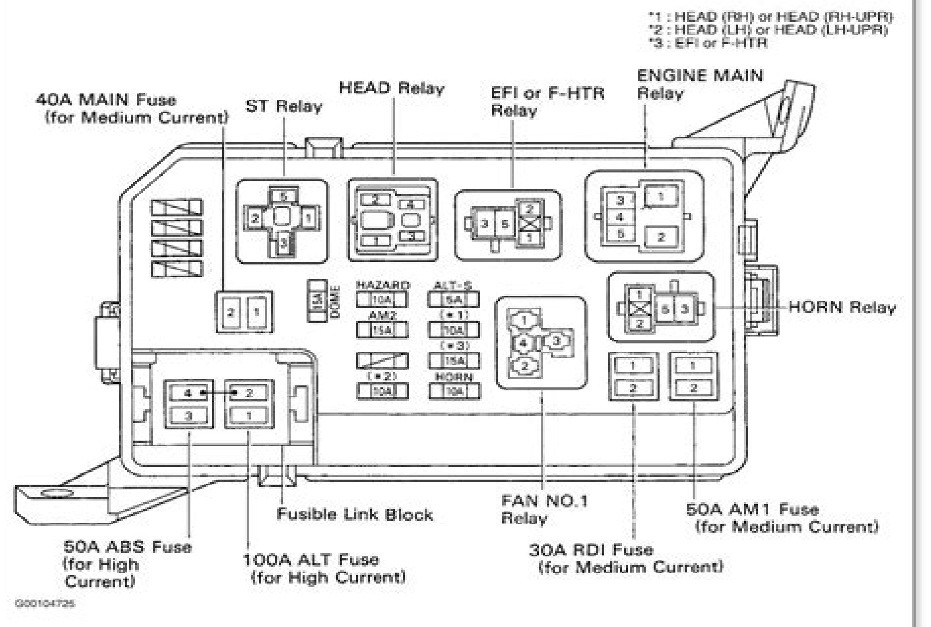
Fig. 15: Identifying Engine Room J/B Components
