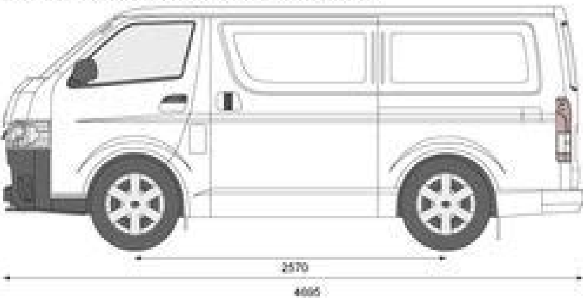
Toyota HiAce H200 LWB Panel Van (2013)
