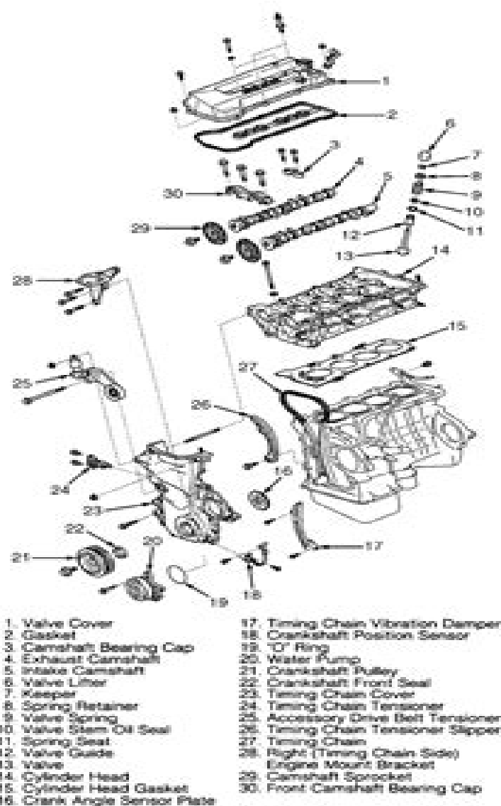
Fig. 6: Exploded View Of Cylinder Head & Timing Chain Components Courtesy of TOYOTA MOTOR SALES, U.S.A., INC.
